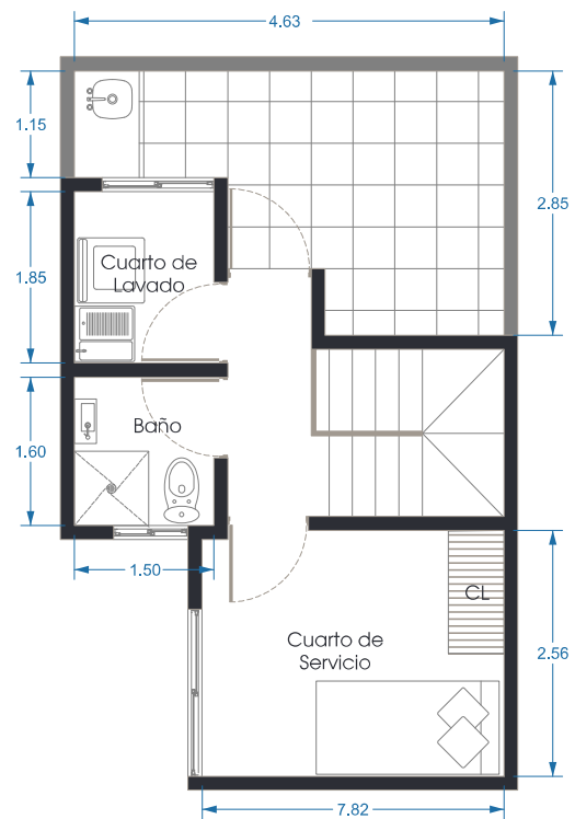
Roof Garden
